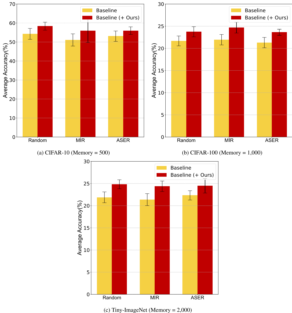
FIGURE 4. Comparison of average accuracy with different retrieval sampling methods across benchmark datasets, including CIFAR-10, CIFAR-100, and Tiny-ImageNet.
