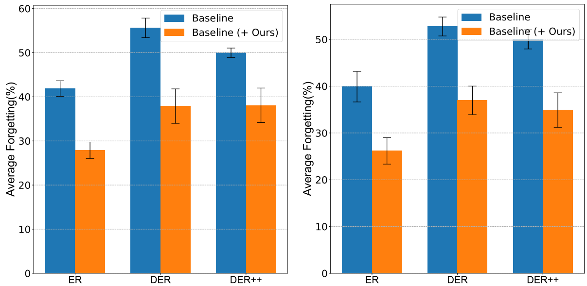
(a) Imbalanced CIFAR-100 (Memory = 1,000)
