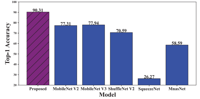
Fig. 1 Top-1 accuracy score of the proposed method and conventional models computed using the CIFAR-10 dataset, where the obtained group structure is H = \{4, 1, 1, 2, 2, 3, 2, 4, 4, 6\}
